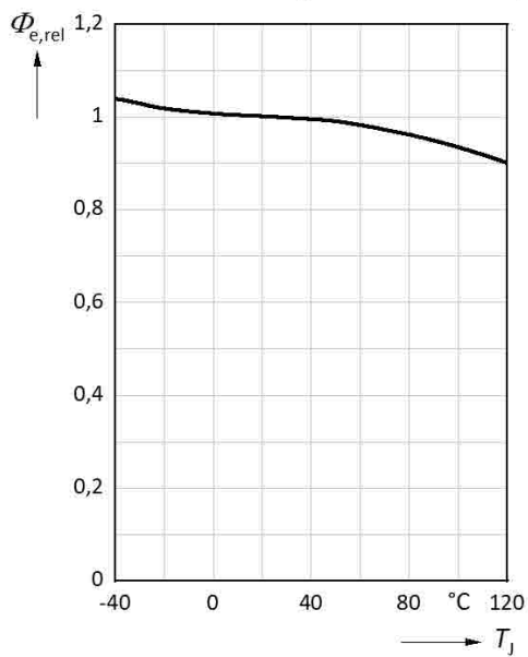
Relative Radiant Intensity vs. Junction Temperature
